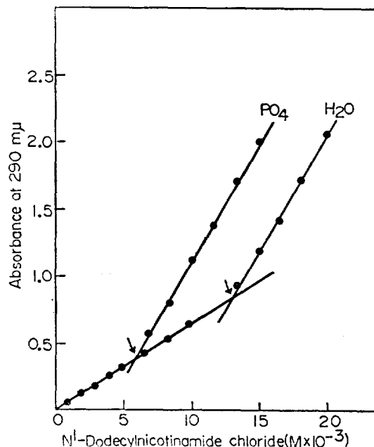
Fig. 3. The spectrophotometric determination of the critical micelle concentration of N 1 -dodecylnicotinamide chloride.
