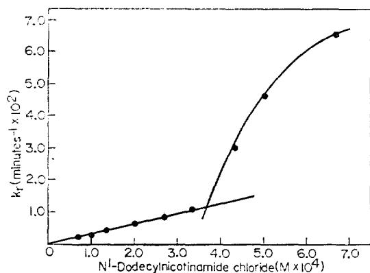
Fig. 2. The effect of N 1 -dodecylnicotinamide chloride concentration on the irreversible inactivation of L- \alpha -glycerophosphate dehydrogenase. Enzyme (2.0 \mu g) was preincubated with varying concentration of DNAC at 15°C in 3.0 ml of 0.05 M tris-HCl buffer, pH 7.85. The residual enzyme activity was expressed by the first order inactivation rate constant ( k_r ) based on Fig. 1.
