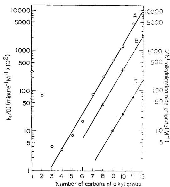
Fig. 8. Chain length effects in reactions of N^1 -alkyl nicotinamide chlorides. Line A represents the values of k_r/[I] against the number of carbons of the inhibitors (see Table 2); Line B, the relationship between the critical micelle concentrations and the chain lengths of the nicotinamide derivative; Line C, the chain length effect on the rates of enzyme inactivation ( k_r ).
