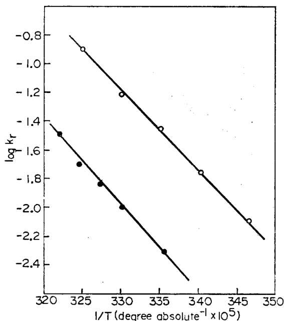
Fig. 7. The Arrhenius plot showing the temperature dependence of L-α-glycerophosphate dehydrogenase inactivation reactions.
