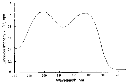
Fig. 2. Excitation spectrum of the aqueous chemiluminescent reagent solution obtained by using the automated stopped flow analyser: [luminol], 1.0 \times 10^{-3} M; [\text{Fe}(\text{CN})_6^{3-}] , 1.0 \times 10^{-2} M; \lambda_{\text{em}} , 412 nm.
