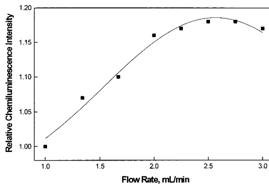
Fig. 6. Effect of flow rate for chemiluminogenic reagent solution on the chemiluminescence intensity to determine glucose using the proposed stopped flow injection system: [luminol], 1.0 \times 10^{-3} M; [glucose], 5.0 \times 10^{-1} mM; \lambda_{em} , 424 nm; flow rate, 3.8 mL/min for P2 streams; volume injected, 2.0 mL for P1 streams and 2.5 mL for P2 streams.
