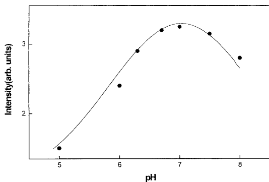
Fig. 4. Effect of pH for the glucose oxidase enzyme reactor on the chemiluminescence intensity: [luminol], 1.0 \times 10^{-3} M; [glucose], 5.0 \times 10^{-1} mM; \lambda_{em} , 424 nm; flow rate, 2.5 mL/min for P1 streams and 3.8 mL/min for P2 streams; volume injected, 2.0 mL for P1 streams and 2.5 mL for P2 streams.
