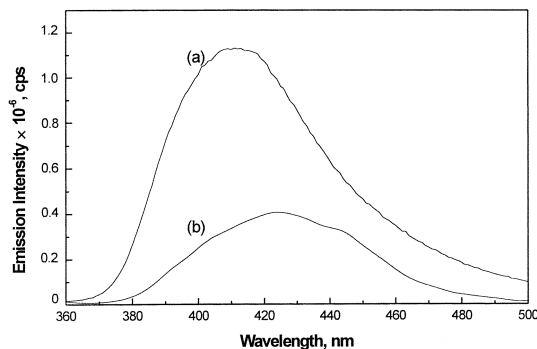
Fig. 3. Emission spectrum of the chemiluminescent reagent solution(a) and chemiluminescence spectrum of the luminol- \text{Fe}(\text{III})\text{-H}_2\text{O}_2 system obtained by using the automated stopped flow analyser(b): [luminol], 1.0 \times 10^{-3} M; [\text{Fe}(\text{CN})_6^{3-}] , 1.0 \times 10^{-2} M in R1 stream; 1.0 \times 10^{-1} M borate buffer solution in R2 stream; [\text{H}_2\text{O}_2] , 1.0 \times 10^{-1} M in R3 stream. R4 stream and enzyme reactor shown in Fig. 1 were not used.
