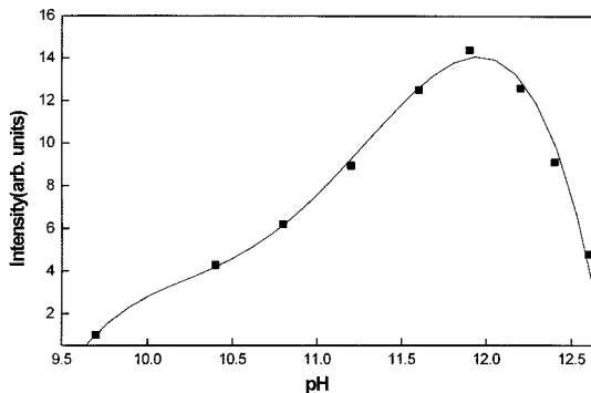
Fig. 5. Effect of pH for 1.0 \times 10^{-1} M borate buffer on the chemiluminescence intensity: [luminol], 1.0 \times 10^{-3} M; [glucose], 5.0 \times 10^{-1} mM; \lambda_{em} , 424 nm; flow rate, 2.5 mL/min for P1 streams and 3.8 mL/min for P2 streams; volume injected, 2.0 mL for P1 streams and 2.5 mL for P2 streams.
