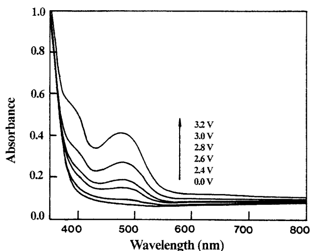
Figure 4. Absorption spectrum of 2,3 dichloro-1,4-napthoquinone, (4a), as a function of the applied electric field. The concentration was 0.196 mM and the path length was 10 mm.
