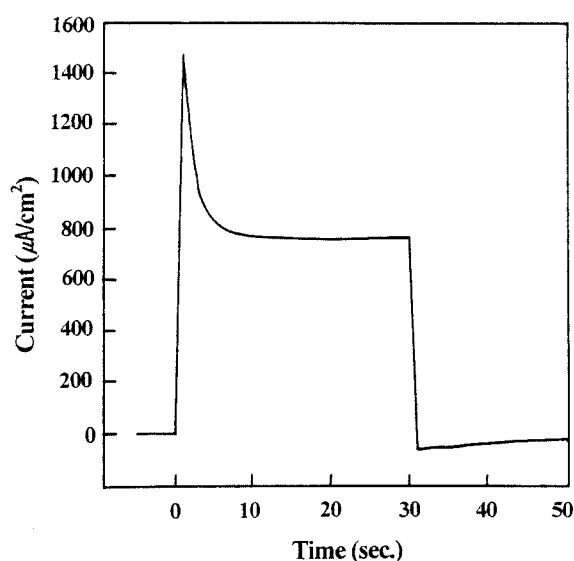
Figure 5. The change in the current with time for 2,3 dichloro-1,4-napthoquinone, (4a). The 3.2V was applied at the time 0 and turned off at 30 seconds.
