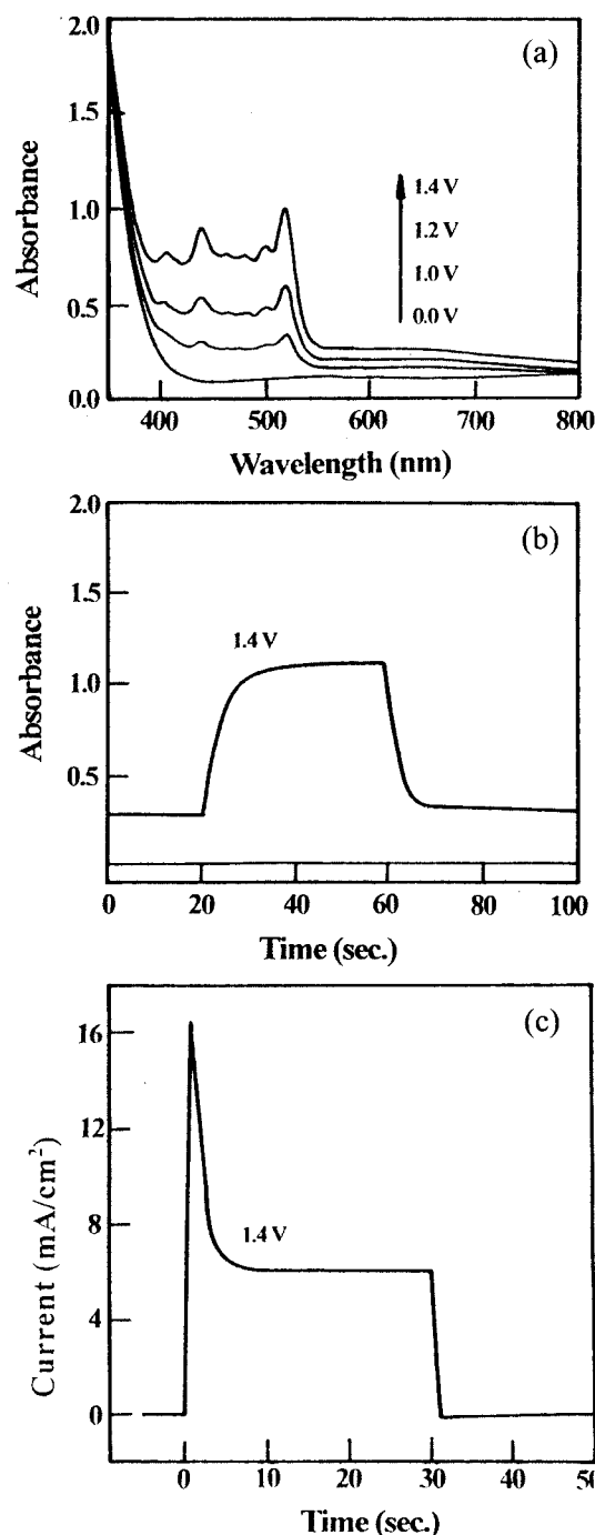
Figure 10. Effect of applied voltage in the absorption pattern (a), change in the absorbance at 510 nm (b), and the current (c). The complex was 1:1 mixture of the 0.098 mM of (3) and (4a).
