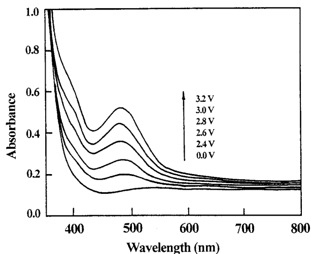
Figure 6. Absorption spectrum of 2,3 dichloro-5-nitro-1,4-napthoquinone, (4b). The conditions are the same as in Figure 4.
