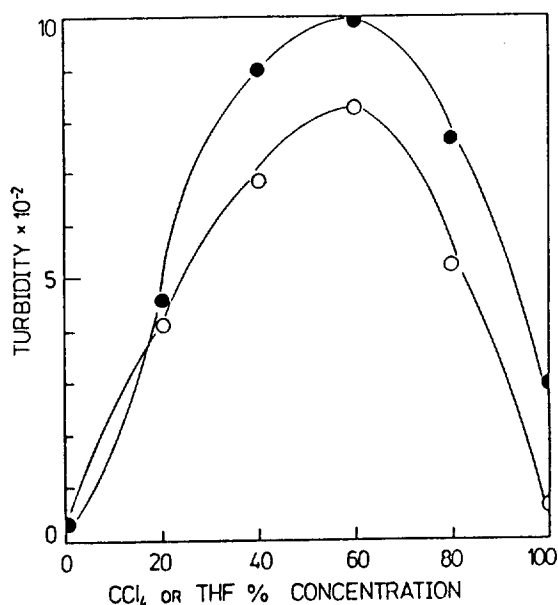
Figure 2. Turbidity change by photopolymerization of acryl amide ( 10^{-1} M) with harmaline ( 5 \times 10^{-4} M) as a function of \text{CCl}_4 (○) or THF (●) % concentration in methanol.
