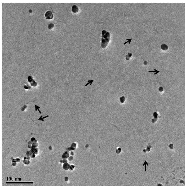
Figure S1. TEM micrograph of exfoliated Ag-laponite nanocomposite after washing prepared in concentrations of \text{AgNO}_3 : 2.5 mmol.
