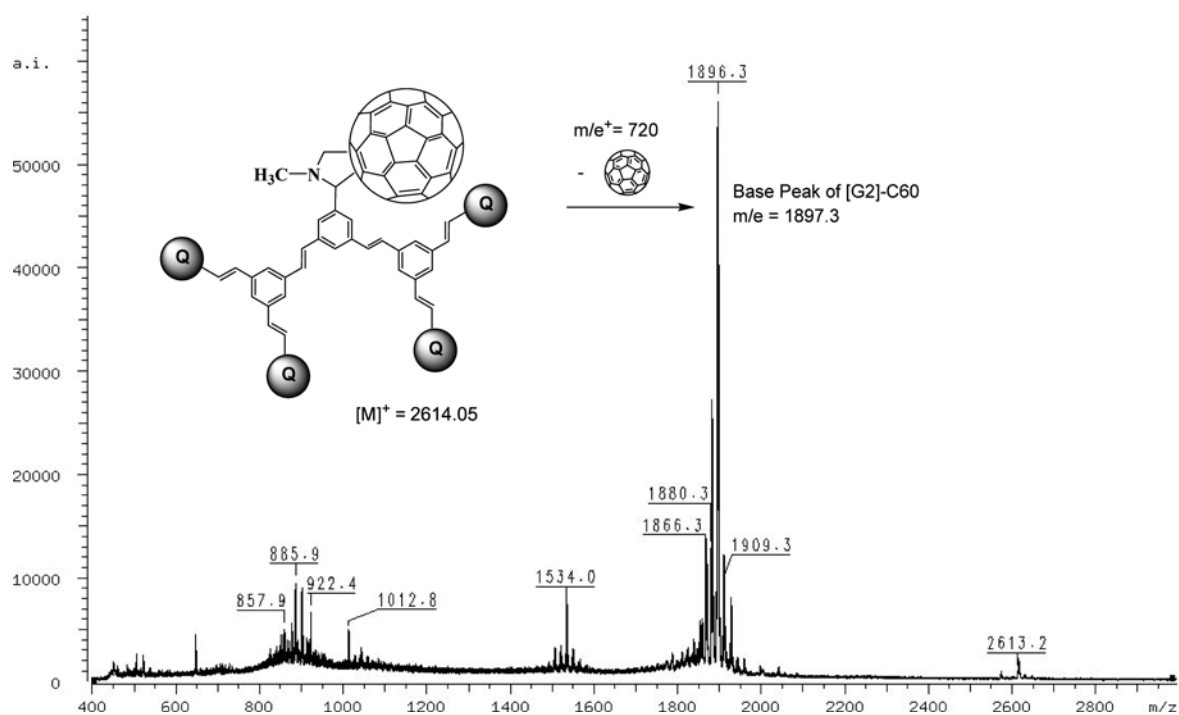
Figure 2. MALDI -TOF spectrum of [G2]-C60 dendron, 2.
