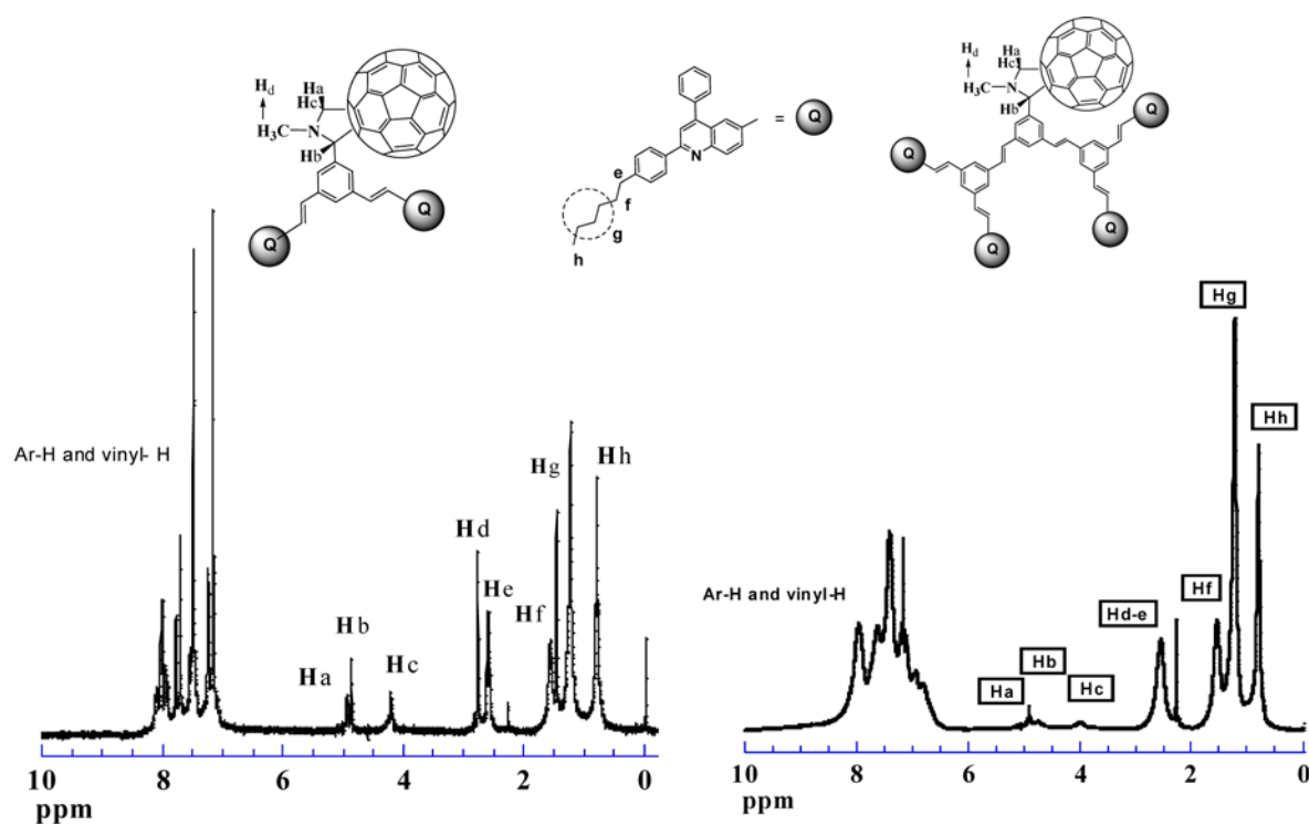
Figure 3. (a) 1 H NMR [G1]-C60 dendron, 1. (b) 1 H NMR [G2]-C60 dendron, 2.
