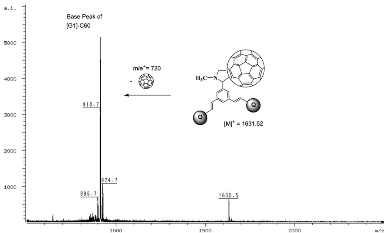
Figure 1. MALDI -TOF spectrum of (a) [G1]-C60 dendron, 1.
