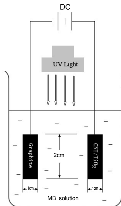
Figure 1. The sketch of EPC decomposition for MB solution with the CNT/TiO 2 electrode.
