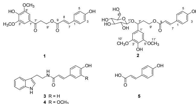
Figure 1. Structures of compounds 1-5 isolated from the leaves of S. quelpaertensis .
